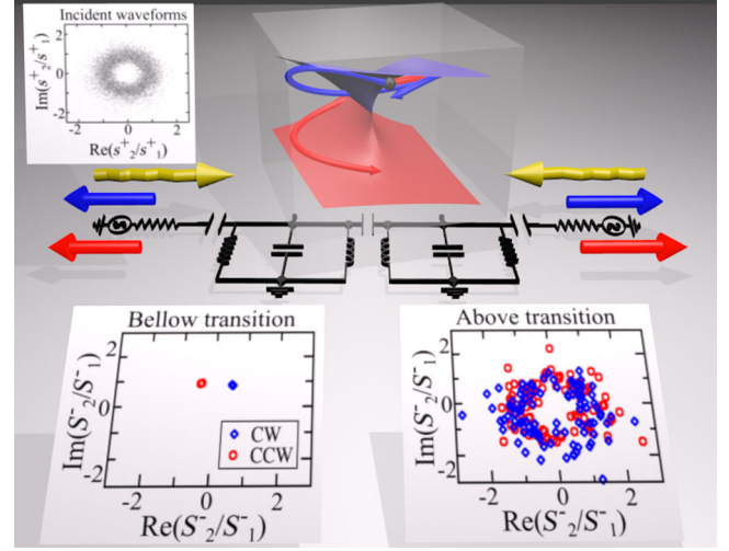
FIG. 3. Electric-circuit scattering setup where a quadiabatic encirclement of an EP degeneracy can lead to a chiral control of the scattered field when the coupling to TLs is smaller than a critical value. The outgoing scattered field, |S_V^-\rangle = (S_1^-, S_2^-)^T , has an attractor determined by the direction of encircling (bottom left). When the coupling to the continuum is large, the outgoing field is sensitive to the specific features of the incident field.
