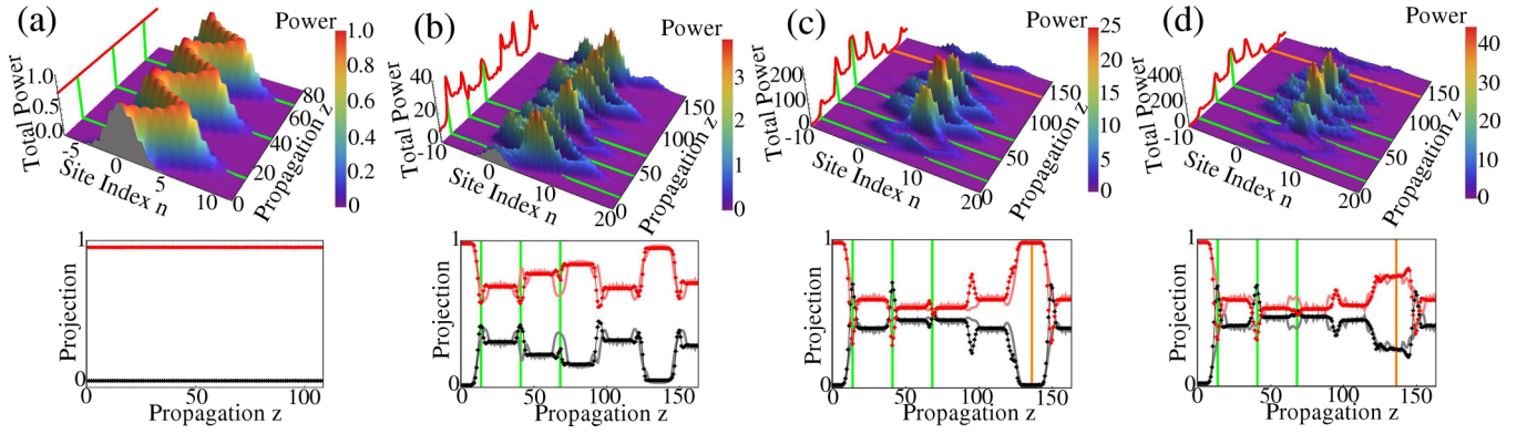
FIG. 3. (Color online) Propagation for an initial Gaussian wave front a_n(0) = b_n(0) = e^{-n^2/10} . The lattice parameters are \alpha = 1 , \omega = 0.231 , and A = 0.6 . The site index n indicates the n th dimer where the amplifying site is juxtaposed with the attenuating site on the right. In the upper subfigures, the red lines show the total power while the color maps describe the individual site power ( |a_n(z)|^2, |b_n(z)|^2 ); the green lines mark the first three Zener distances z_Z while the orange lines mark the expected self-imaging time z_{SI} (approx. at 136). In the lower graphs the gray and pink lines correspond to the normalized relative band-power evaluated numerically from the beam evolution (see text). The black and red dots correspond to the upper and lower band projections [Eq. (9)], normalized to the total power at each distant z . In (a) \gamma = 0 , in (b) \gamma = 0.405 , while in (c) and (d) \gamma = 0.443 . In (d) a defect is included in the seventh dimer during the propagation interval z \in [z_Z^{(1)} - 4, z_Z^{(1)} + 4] (see text for details). The presence of the defect disrupts the expected revival at z_{SI} [see the lower subfigure (c) where the expected z_{SI} (approx. at 136) is marked with an orange line] and results in a huge total power at the recombination distance z_R [third green line at upper subfigure (d)]. The behavior of subfigures (b)–(d) is typical and has been observed over a wide range of the parameter A .
