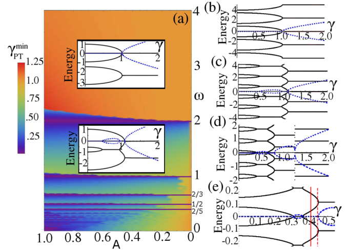
FIG. 2. (Color online) Numerical results for (a) the first EP of the system for \alpha = 1 , versus \omega and A ; (b–d) The real (black) and imaginary (blue dotted) spectra in domains 1, 2, 3 for A = 0.5 and \alpha = 1 . In (b) \omega = 2.5 , in (c) \omega = 1.5 , and in (d) \omega = 0.85 . (e) Spectrum for A = 0.6 and \omega = 0.231 associated with the parameters used in Fig. 3. The perpendicular solid (dashed) lines indicate the values of \gamma = 0.405 ( \gamma = 0.443 ) associated with Figs. 3(b) and 3(c). The subfigures in (a) are plots of Eqs. (5) and (6), respectively, for the same parameters as (b) and (c). The purple lines indicate the \omega_m values separating domains with different numbers of instability regions (see text).
