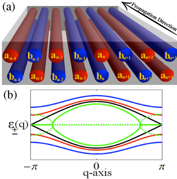
FIG. 1. (Color online) (a) Photonic lattice (for \omega = 0 ) with \mathcal{P}_d\mathcal{T} symmetry [26]. Red (blue) waveguides indicate waveguides with amplification (attenuation) [21]. (b) Associated dispersion relation for \gamma = 0 (outer blue lines for upper and lower bands), 0 \leq \gamma \leq \gamma_{PT} (upper and lower red lines before the blue outer ones), \gamma = \gamma_{PT} (upper and lower black lines before the blue ones which are associated with the EP degeneracy at q = \pm\pi ), and the solid (dashed) green (inner) lines are the real (imaginary) part for \gamma > \gamma_{PT} .
